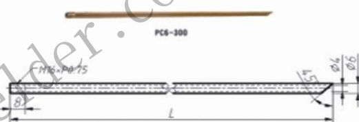
耐热冷却水管(Tube For Cooling) (TEFLON)
