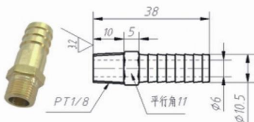
直通水接头(Hose Connector) (BSBM) FG-1/8
