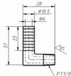
水冷铜管(Pipe For Cooling) (Cu)
