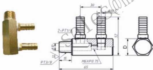
直通水接头(Hose Connector) (BSBM) FG-1/8
